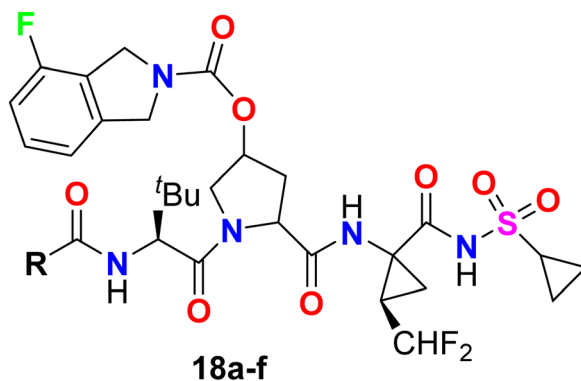
Fig. 13 Structure of 4-fluoroisoindoline derivatives 18a–f .
