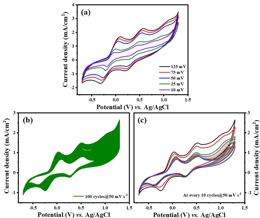
Fig. 6 (a) \text{Ti}_3\text{C}_2\text{T}_x\text{-PTh} at various scan rates (b) and (c) stability test of \text{Ti}_3\text{C}_2\text{T}_x\text{-PTh} at 50 mV s -1 for 100 cycles and plotted at every 10 cycles.
