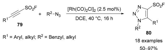
Scheme 28 Synthesis of alkynyl sulfonyl fluoride reagents 79 and application for synthesis of 4-sulfonyl fluoride-substituted triazoles 80 .
