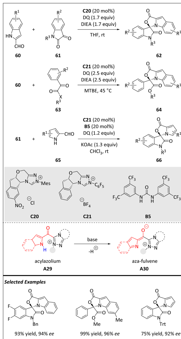
Scheme 21 Enantioselective intermolecular [10 + 2] cycloadditions via the 10π aza-fulvene intermediate.
