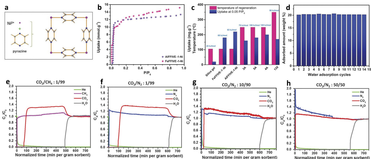
Fig. 18 (a) The repetitive square pattern in the Ni-pyrazine (4,4') square-grid layer. (b) Water adsorption isotherms of AIFVIVE-1-Ni (violet) and FeFFVIVE-1-Ni (pink) at 35 °C. (c) Comparison and relationship between water uptake at P/P_0 = 0.05 , heat of sorption, and regeneration temperature of AIFVIVE-1-Ni and FeFFVIVE-1-Ni, along with commercial desiccants. (d) Cycles for water adsorption uptake of AIFVIVE-1-Ni (adsorption at 25 °C and desorption at 105 °C). (e) Breakthrough test with a humid (75% RH) CO 2 /CH 4 : 1/99 mixture. (f)–(h) Effect of CO 2 concentration on water breakthrough tests (humid 75% RH). Reproduced with permission from ref. 20. Copyright, 2017, The American Association for the Advancement of Science.
