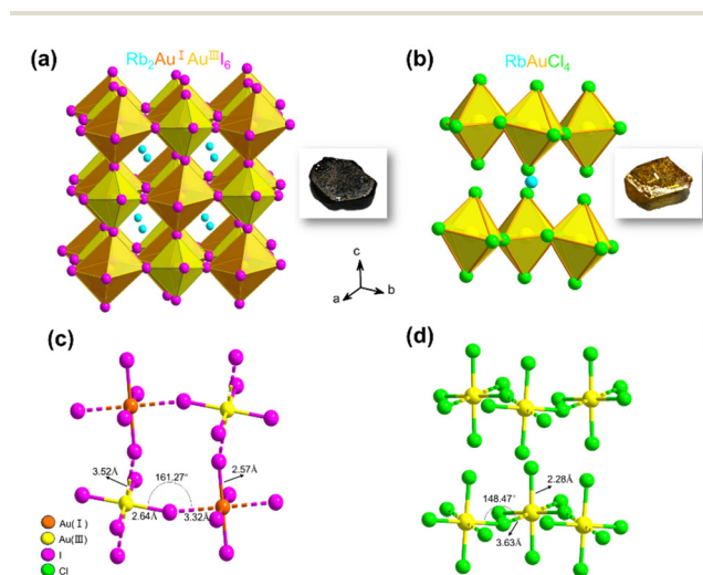
Fig. 1 Single-crystal X-ray diffraction analysis of (a) Rb 2 Au 2 I 6 and (b) RbAuCl 4 . The blue, orange, gold, red, purple, and green spheres represent Rb, Au I , Au III , I, and Cl atoms, respectively. The insets show the photographs of the crystals. (c and d) Bond lengths and angles of Rb 2 Au 2 I 6 and RbAuCl 4 . Rb atoms are omitted in the schematic diagram for the ease of structural description.
