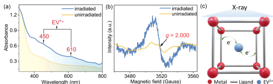
Fig. 4 Radiochromic mechanism for RCS-2 : (a) electronic absorption spectra before and after irradiation. (b) EPR spectra before and after irradiation. (c) Schematic diagram of the electron transfer mechanism.
