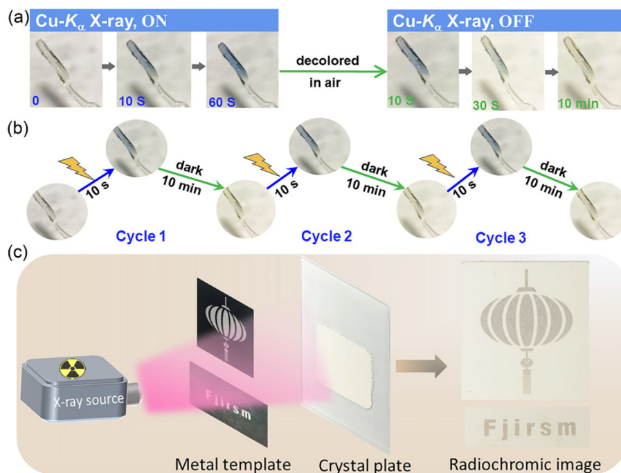
Fig. 3 Radiochromic behavior for RCS-2 : (a) time-dependent images for crystalline samples of RCS-2 upon irradiation of \text{Cu-K}\alpha X-rays. (b) Colored-decolored cycles of a single-crystal sample upon irradiation of \text{Cu-K}\alpha . (c) Radiochromism imaging. (The photographs of (a) and (b) were both captured in their original context.)
