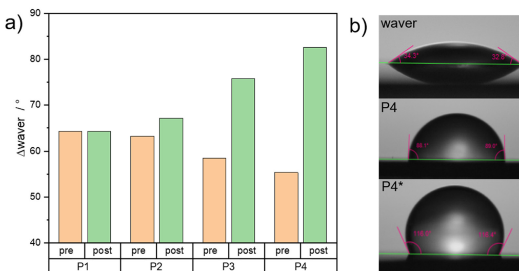
Fig. 5 Water contact angle results of spin-coated polymer on silica wavers for synthesized polymers PS_{797}\text{-}b\text{-(PtBAEMA}_{21}\text{-co-PMMA}_6\text{)} (P1), PS_{773}\text{-}b\text{-(PtBAEMA}_{45}\text{-co-PMMA}_{13}\text{)} (P2), PS_{773}\text{-}b\text{-(PtBAEMA}_{71}\text{-co-PMMA}_{23}\text{)} (P3) and PS_{776}\text{-}b\text{-(PtBAEMA}_{108}\text{-co-PMMA}_{37}\text{)} (P4) with respective functionalized counterparts; (a) Compiled results for water contact angle measurements before and after functionalization of the silica wavers; (b) Exemplary photographs for water contact angle measurements for P4 and P4*.
