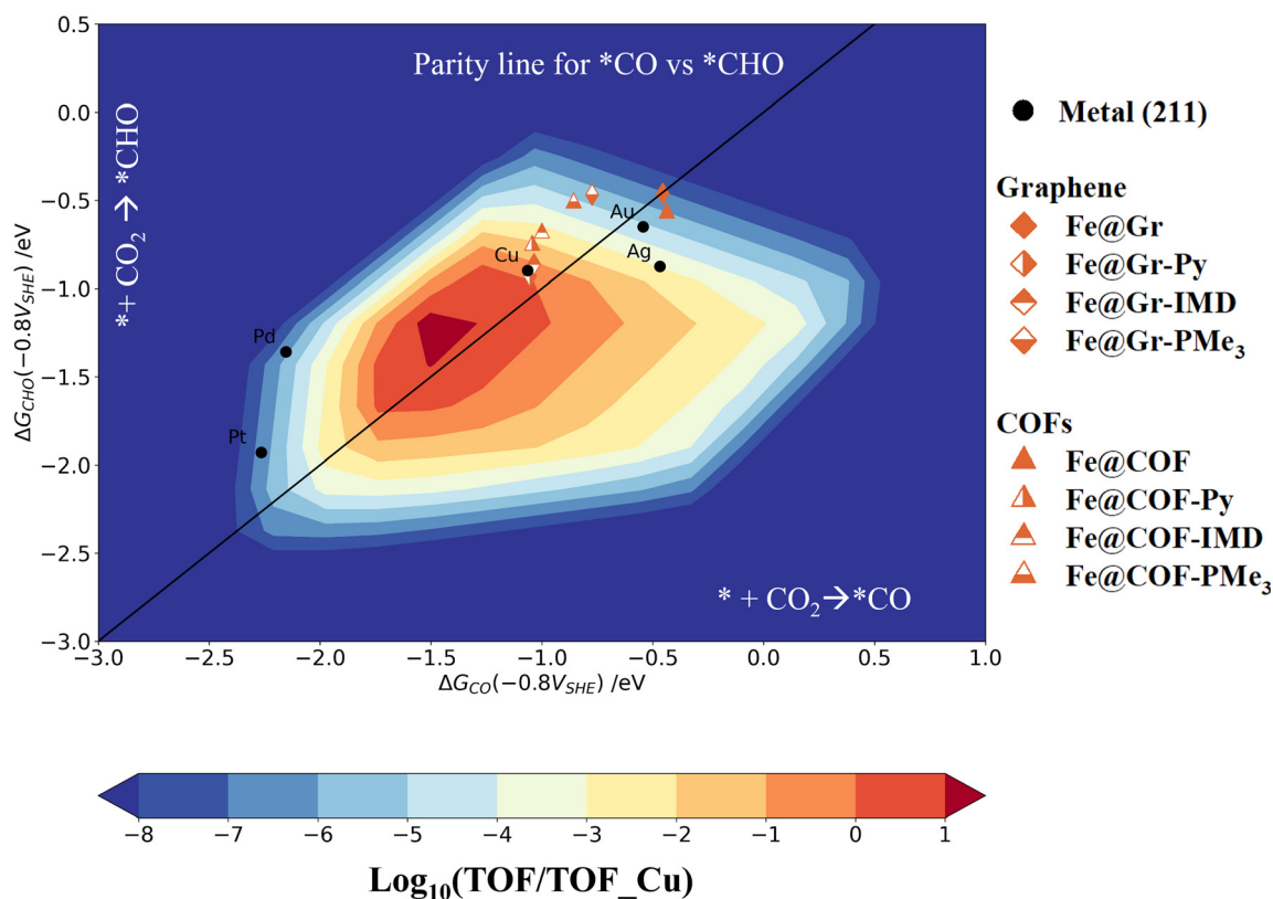
Fig. 6 Unified activity volcano plot for CO 2 → CH 3 OH/CH 4 formation, plotted using the free energies of \text{*CO} and \text{*CHO} intermediates as the activity descriptors at an applied potential of -0.8 V vs. SHE and pH of 6.8. The Fe@Gr/COF catalysts with and without axial ligands are represented using different markers, as shown in the right inset of Fig. 6. The catalytic activity is shown on a logarithmic scale with respect to the Cu (211) surface. The black circles represent the activity of the 211 surfaces of Pt, Pd, Au, Ag, and Cu. The parity line denoted by a black solid line indicates the preference for PDS between the \text{*} + \text{CO}_2 \rightarrow \text{*CO} and \text{*} + \text{CO}_2 \rightarrow \text{*CHO} intermediates. The activity with respect to the Cu (211) surface increases on moving from blue to red regions. Without the axial ligands, both Fe@Gr and Fe@COF show similar activity to that of the Au (211) surface. With the different axial ligands, the SACs show activity comparable to that of Cu (211) surfaces.
