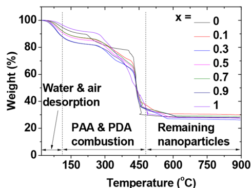
Fig. 4 TGA curves of \text{GdEu}_x\text{Tb}_{1-x}\text{O}_3@PAA/PDA nanoparticles ( x = 0, 0.1, 0.3, 0.5, 0.7, 0.9 , and 1 ) under air flow.
