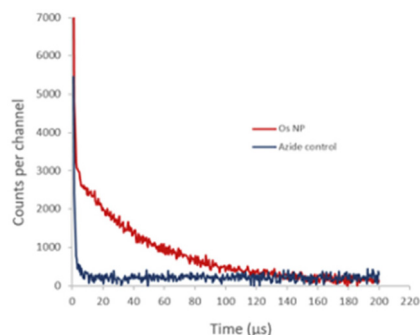
Fig. 7 Time-resolved singlet oxygen NIR phosphorescence decays from OsPhenSS-AuNP13 in D 2 O 4.5 nM ( \lambda_{\text{det}} = 1270 \pm 20 nm). Red: without the addition of azide; blue: with the addition of azide (5 mM). The initial short-lived signal is due to the residual NIR tail of fluorescence from the osmium signal. In the presence of azide, which is a physical quencher of singlet oxygen, the NIR phosphorescence tail is suppressed.
