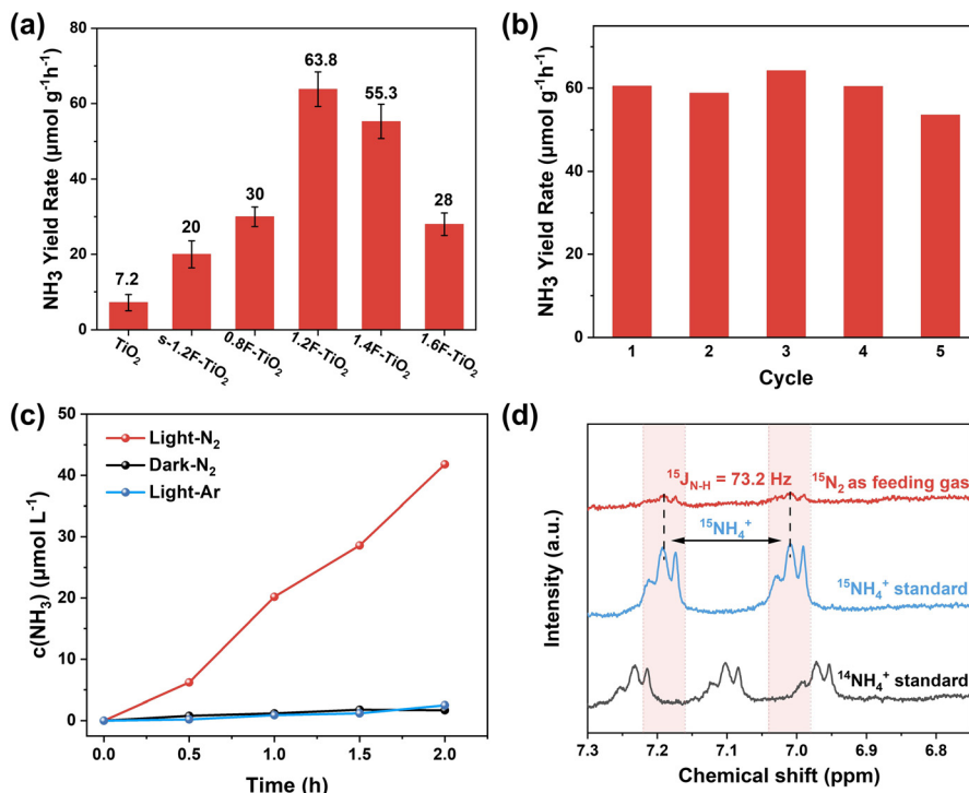
Fig. 3 (a) Photocatalytic ammonia yield rates of \text{TiO}_2 , \text{s-1.2F-TiO}_2 and \text{xF-TiO}_2 . (b) Recycling experiments of \text{1.2F-TiO}_2 . (c) \text{NH}_3 production versus time over \text{1.2F-TiO}_2 with various reaction conditions. (d) The ^1\text{H} NMR spectra of \text{1.2F-TiO}_2 bubbled with a ^{15}\text{N}_2 atmosphere.
