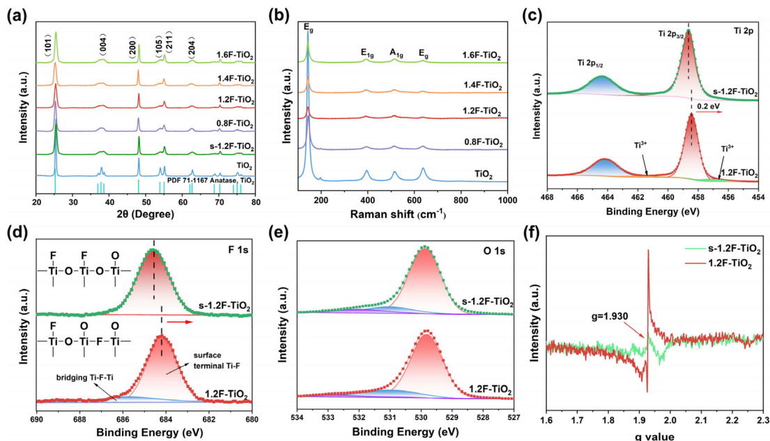
Fig. 2 (a) XRD patterns of \text{TiO}_2 , \text{s-1.2F-TiO}_2 and \text{F-TiO}_2 . (b) Raman spectra of \text{TiO}_2 and \text{F-TiO}_2 . (c) Ti 2p, (d) F 1s, (e) O 1s XPS, and (f) EPR spectra of \text{s-1.2F-TiO}_2 and \text{1.2F-TiO}_2 .
