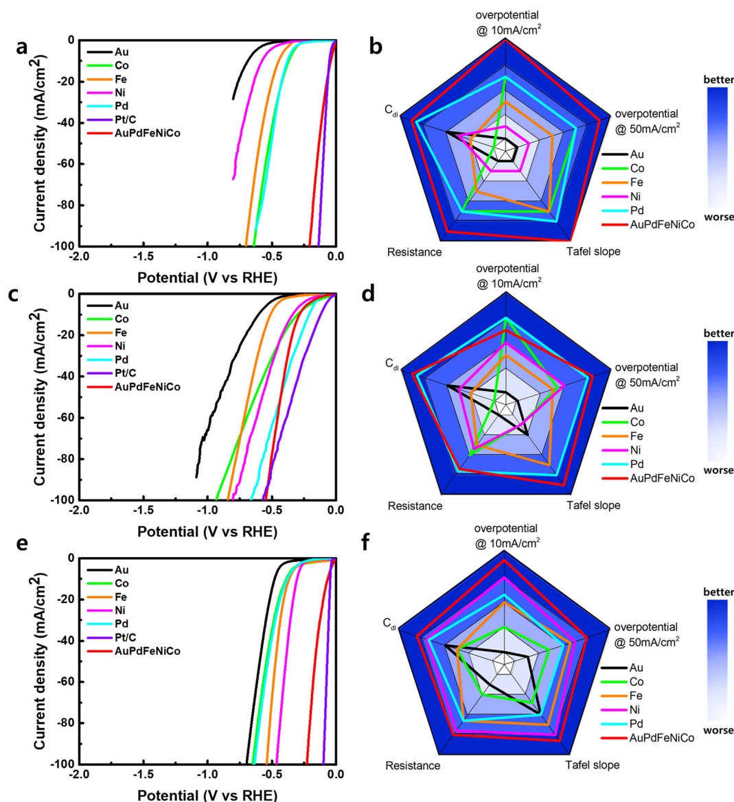
Fig. 4 HER electrocatalysis in acidic, neutral, and alkaline electrolyte. HER polarization curves of Au, Pd, Fe, Ni, Co, AuPdFeNiCo, and Pt/C in (a) 0.5\text{M H}_2\text{SO}_4 , (c) 1\text{M PBS} , (e) 1\text{M KOH} , corresponding radar chart comparison of the potential characteristics of the electrocatalysts in (b) 0.5\text{M H}_2\text{SO}_4 , (d) 1\text{M PBS} , and (f) 1\text{M KOH} .
