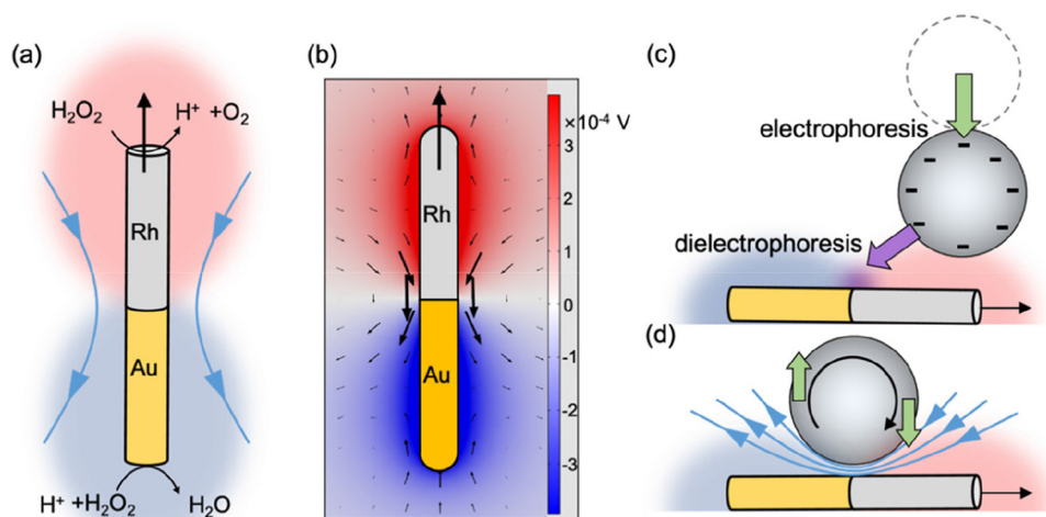
Fig. 3 The mechanism of the collection and spinning of SiO 2 -Au Janus microspheres by an Au-Rh nanorod motor. (a and b) Schematic diagram (a) and numerical simulation (b) of the electric potential (colors) and fluid flows (arrows) around an Au-Rh nanorod in the lab frame. The sizes of the arrows are proportional to the flow magnitude. (c) Schematic of a negatively charged SiO 2 -Au Janus microsphere being collected to a nanorod motor via the combined effect of electrophoresis and dielectrophoresis. (d) Schematic of a negatively charged SiO 2 -Au Janus microsphere spinning near a nanorod motor via torques produced by electrostatics (green arrows) and flows (blue arrows).
