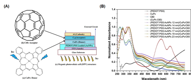
Fig. 11 (A) Chemical structure of CuPc as a donor (a) and fullerene (C60) as an acceptor (b), and schematic structure of the organic photovoltaic cell (c); (B) normalized absorption spectra of CuPc, C60, and different sizes of AuNSs embedded in PEDOT:PSS/CuPc/C60 multilayer films. Reproduced from ref. 50 with permission from Elsevier (CC BY-NC 4.0).
