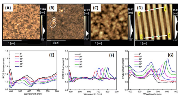
Fig. 24 AFM images of HTL films prepared from (A) PEDOS:PSS and (B) G-AuQD-loaded PEDOT:PSS. The white circles in (B) indicate the domains of aggregated G-AuQDs. AFM images of the (C) flat and (D) BD-R imprinted photoactive layers. (E–G) Spectra depicting the enhancement of IPCE for green-AuQD/BD-R OSCs under non-polarized light irradiation at different angles of incidence. The figures represent the IPCE enhancement spectra for (E) G-AuQD OSC, (F) BD-R OSC, and (G) G-AuQD/BD-R OSC. Reproduced from ref. 110 with permission from the Royal Society of Chemistry (CC BY-NC 4.0).
