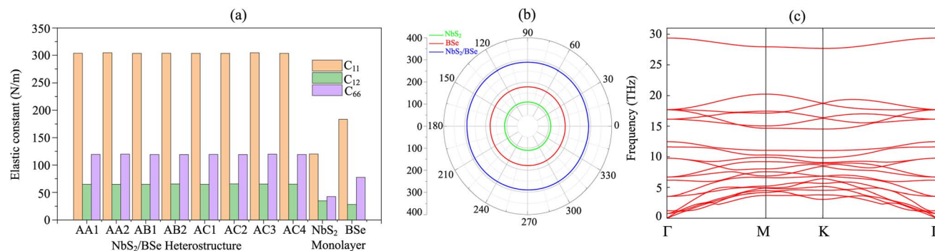
Fig. 3 (a) Calculated independent elastic constants ( C_{ij} ) of the \text{NbS}_2/\text{BSe} heterostructure for different stacking configurations and (b) angle-dependent Young's modulus and (c) phonon dispersion curves of the \text{NbS}_2/\text{BSe} heterostructure for the most energetically favorable stacking configuration.
