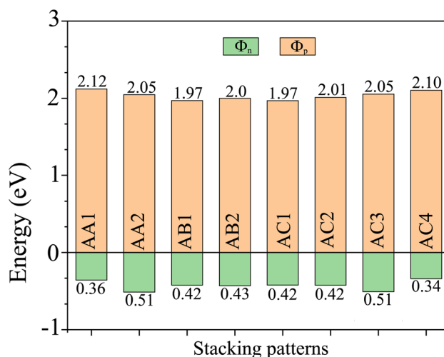
Fig. 5 The Schottky barriers of the \text{NbS}_2/\text{BSe} heterostructure for different stacking patterns.
