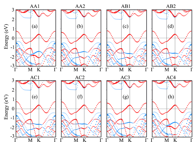
Fig. 4 Projected band structures of the \text{NbS}_2/\text{BSe} heterostructure for different stacks of (a) AA1, (b) AA2, (c) AB1, (d) AB2, (e) AC1, (f) AC2, (g) AC3 and (h) AC4. Red and blue bubbles represent the contributions of the \text{NbS}_2 and \text{BSe} layers, respectively.
