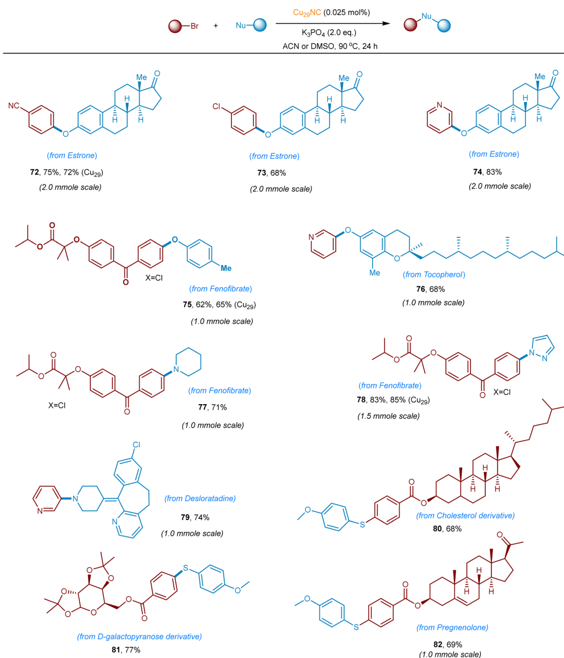
Fig. 10 Late-stage functionalization of complex organic and drug molecules. Standard reaction conditions. Yield of isolated product after purification by column chromatography on a silica gel. (Cu29-S) indicates heterogeneous Cu 29 -Celite S.
