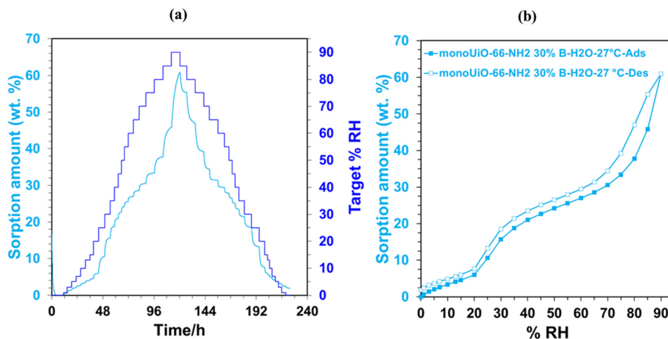
Fig. 7 DVS plots for \text{monoUiO-66-NH}_2\text{-30%-B} ; (a) kinetic plot and, (b) water sorption isotherm.
