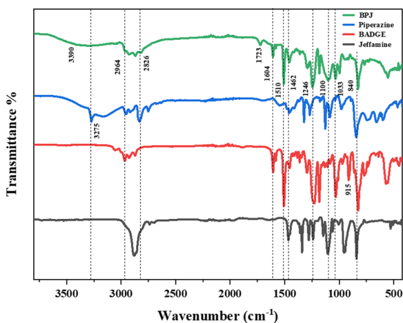
Fig. 1 FTIR spectrum of BPJ polymer.
