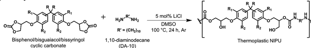
Scheme 1 Synthesis of (a) BGF/BSF using guaiacol/syringol and vanillyl/syringyl alcohol, (b) BGA/BSA using guaiacol/syringol and acetone, (c) diglycidyl ether of bisguaiacol/bisysyringol from respective bisguaiacol/bisysyringol and epichlorohydrin, (d) bisguaiacol/bisysyringol cyclic carbonate from respective diglycidyl ether and \text{CO}_2 , and (e) NIPU using respective bisguaiacol/bisysyringol cyclic carbonate and 1,10-diaminodecane (DA-10).
