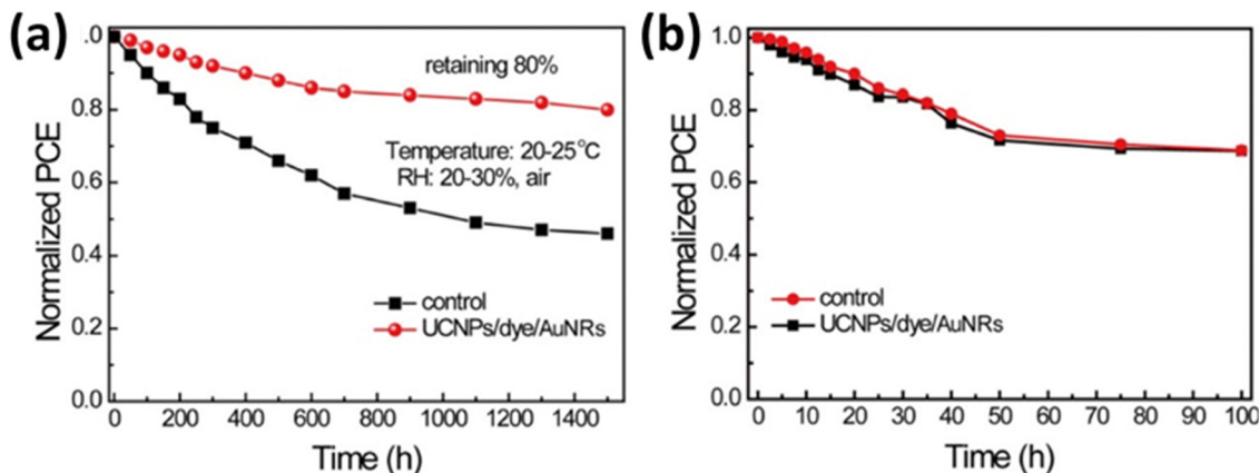
Fig. 17 (a) The stability of devices for a control film and a film incorporating a UCNP/IR-783 dye/AuNRs composite film under an air environment, RH = 20–30% and 20–25 °C. (b) Light stability of devices for a control film and a film incorporating a UCNP/IR-783 dye/AuNRs composite under AM 1.5G irradiation. Reprinted with permission from the American Chemical Society. 74
