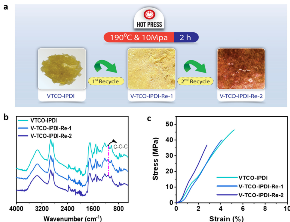
Fig. 8 (a) Recycling by hot pressing. (b) FTIR spectra of reprocessed VTGO-IPDI. (c) Stress-strain curves of reprocessed VTGO-IPDI.
