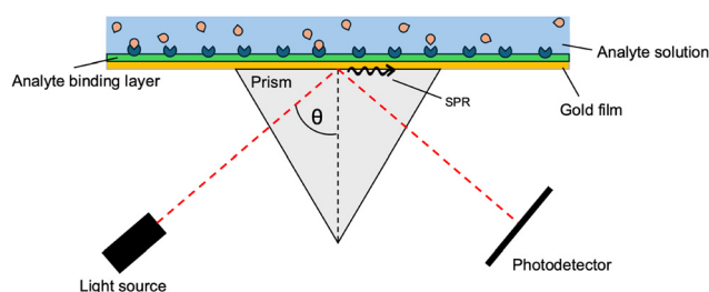
Fig. 2 Depiction of the SPR sensor technology in a Kretschmann configuration. A specific angle of reflectance will instigate SPR, causing a decrease in measured light intensity. As the analyte binds, the angle at which SPR occurs will shift. This figure was created by the authors.
