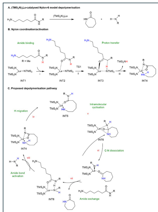
Fig. 8 Mechanistic illustration of Nylon-6 depolymerisation with commercially available lanthanide trisamido catalysts \text{Ln}(\text{N}(\text{TMS})_2)_3 (Ln = lanthanide). (A) Computed Nylon-6 model reaction. (B) Nylon coordination. (C) Proposed depolymerisation mechanism. Reproduced from ref. 175 with permission from Wiley, copyright 2023.
