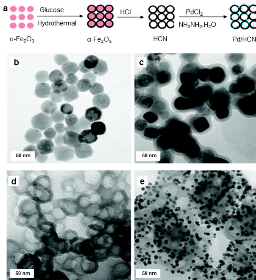
Fig. 7 (a) Schematic illustration of synthesis of the Pd/HCN catalysts; (b–e) TEM images of \alpha - \text{Fe}_2\text{O}_3 NPs, \alpha - \text{Fe}_2\text{O}_3 @C, HCN, and Pd/HCN catalysts respectively. Reproduced with permission from ref. 131 Copyright 2013, The Royal Society of Chemistry.
