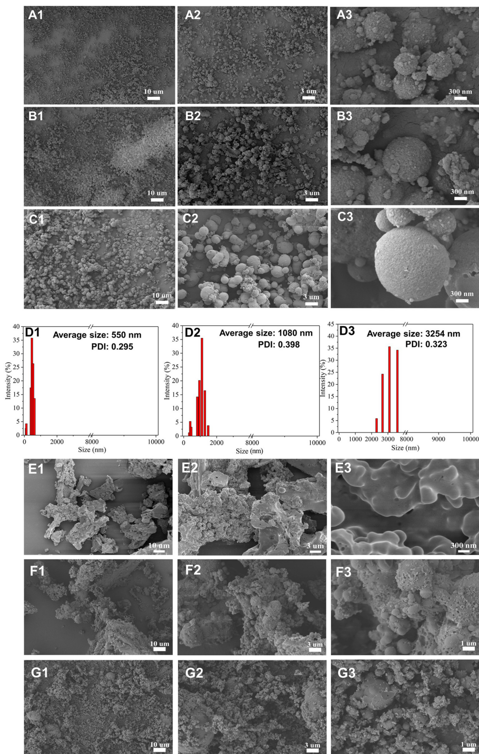
Fig. 2 SEM images of isolated LMPs and their size distribution. (A1–A3) Images of L GLDES ; (B1–B3) L EGDES and (C1–C3) L BDES ; and the size distributions of (D1) L GLDES , (D2) L EGDES and (D3) L BDES ; (E1–E3) morphology of CEL and lignins isolated from organic acid-based DES systems of (F1–F3) LADES and (G1–G3) OADES.
