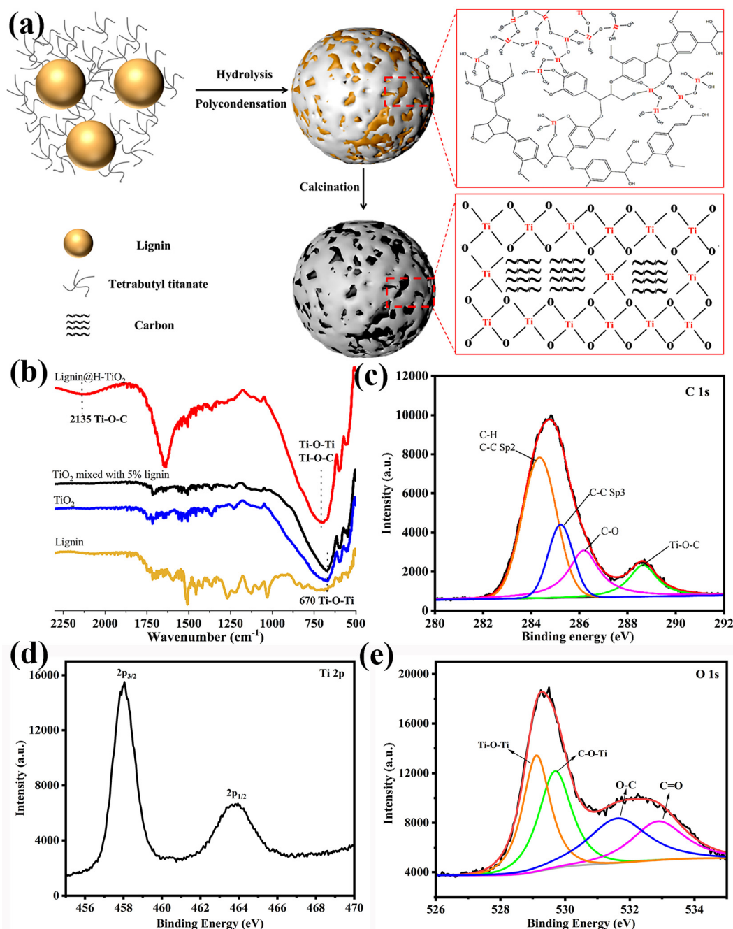
Fig. 1 (a) Schematic illustration of the C lignin @H-TiO 2 synthetic procedure. (b) FTIR of lignin@H-TiO 2 , TiO 2 mixed with 5% lignin, TiO 2 and lignin. XPS spectra of (c) C 1s, (d) Ti 2p and (e) O 1s for lignin@H-TiO 2 .
