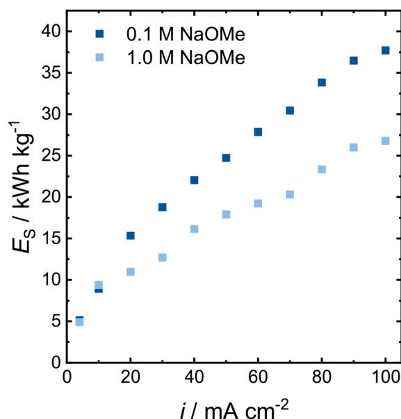
Fig. 7 Specific energy consumption for the formaldehyde synthesis in NaOMe on a 12 \text{ cm}^2 Pt electrode in an electrochemical flow cell at 100 \text{ mL min}^{-1} .
