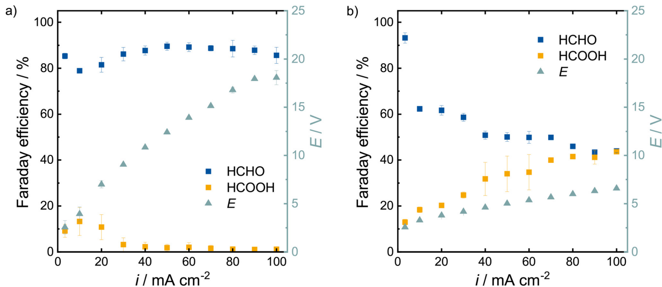
Fig. 6 Faraday efficiency for formaldehyde and formic acid and the required potential for different current densities on Pt in (a) 0.1 \text{ mol L}^{-1} and (b) 1.0 \text{ mol L}^{-1} NaOMe in MeOH at a flow rate of 100 \text{ mL min}^{-1} after 30 min.
