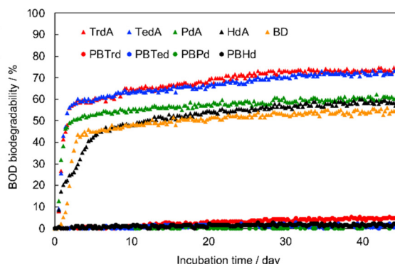
Fig. 13 BOD biodegradation curves of 1,4-butanediol (BD), n -alkylene dicarboxylic acid (DCAs), including tridecanoic diacid ( n = 11; TrdA), tetradecanoic diacid ( n = 12; TedA), pentadecanoic diacid ( n = 13; PdA), and hexadecanoic diacid ( n = 14; HdA), and PBADs at 25 °C for 45 days. Reproduced from ref. 92 with permission from Elsevier, copyright 2021.
