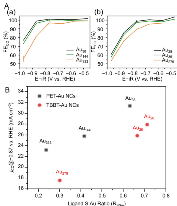
Fig. 19 (A) FE CO of (a) PET-protected Au 38 , Au 144 and Au 333 and (b) TBBT-protected Au 28 , Au 36 and Au 279 NCs. (B) Electrochemical performance: j_{\text{CO}} (at -0.87 V vs. RHE) vs. S: Au ratio of Au 38 , Au 144 , Au 333 and Au 28 , Au 36 , Au 279 series of NCs (A) and (B) are reproduced with permission from ref. 296. Copyright 2022 Wiley-VCH GmbH.
