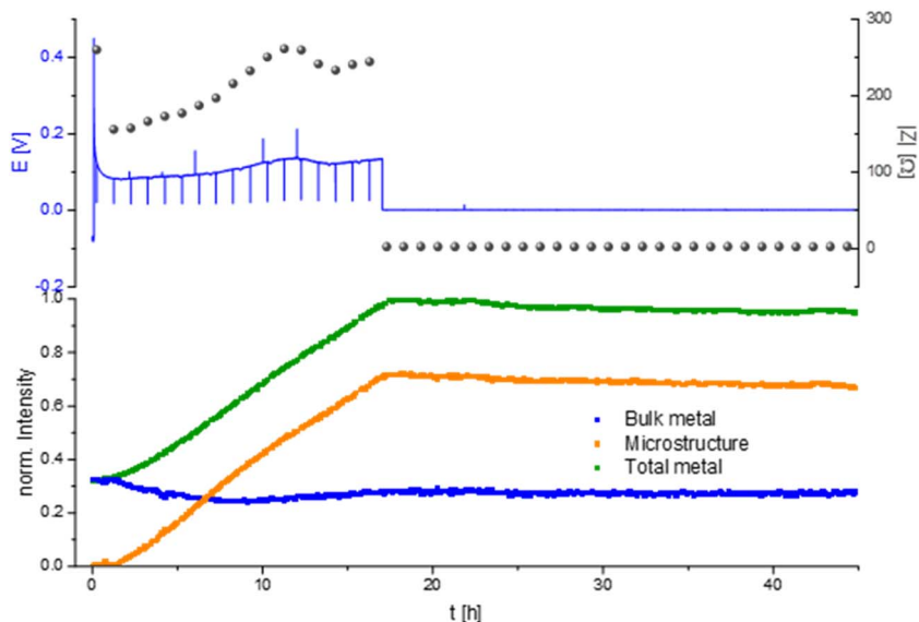
Fig. 8 Operando ^7\text{Li} NMR and impedance (GEIS) measured at 8 Hz intensities measured during unidirectional Li plating at 1\text{ mA cm}^{-2} in an NMR in situ cylindrical symmetrical Li cell with LP30 electrolyte.
