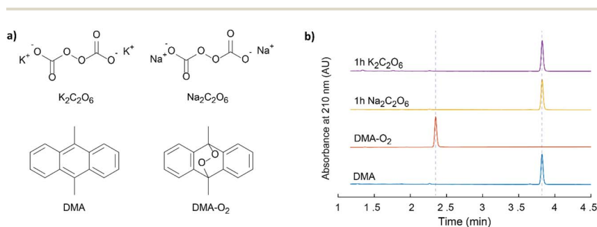
Fig. 3 (a) The structures of the symmetric Na and K peroxydicarbonates, DMA and DMA- \text{O}_2 . (b) HPLC elugrams of these peroxydicarbonates in contact with 30 mM DMA in DME together with reference elugrams of DMA and DMA- \text{O}_2 .
