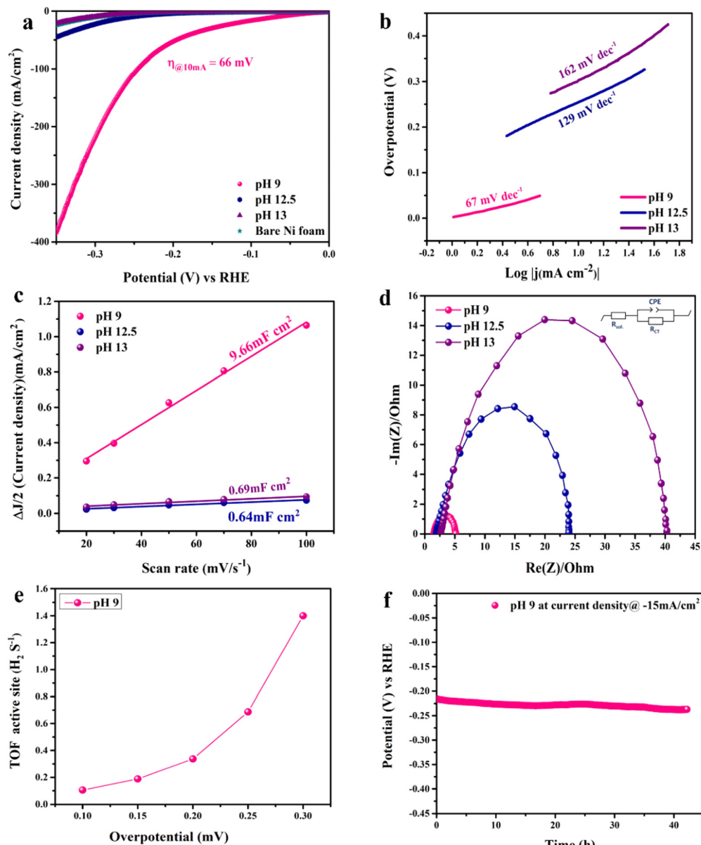
Fig. 5 HER activity of the \text{CoFe}_2\text{O}_4/\text{Ni} foam catalysts in 1 M KOH: (a) iR-corrected LSV plots at a scan rate of 10 \text{ mV s}^{-1} , (b) Tafel slopes of the catalysts, (c) double layer capacitance used to determine the ECSA of all catalysts, (d) Nyquist plots at -0.176 \text{ V (RHE)} in the 1 \text{ mHz} - 100 \text{ KHz} frequency range with the inset representing the fitted equivalent Randle's circuit, (e) TOF over a wide range of potentials for the catalyst prepared at pH 9, and (f) the chronopotentiometry durability test performed at -15 \text{ mA cm}^{-2} for the material prepared at pH 9.
