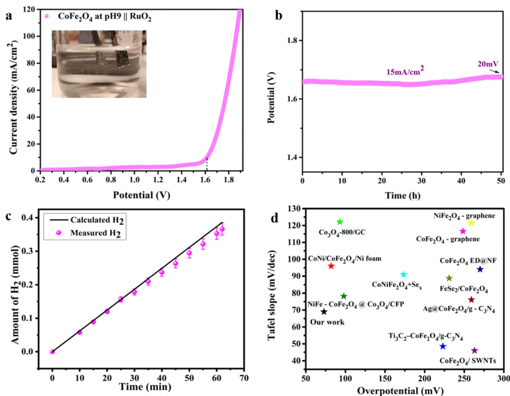
Fig. 6 The overall water splitting electrolyzer performance determined using the pH 9 \text{CoFe}_2\text{O}_4 electrocatalyst as the cathode and \text{RuO}_2 as the anode in 1 M KOH solution. (a) iR-compensated LSV plot at a 10 \text{ mV s}^{-1} scan rate, (b) CP durability test recorded at 15 \text{ mA cm}^{-2} , (c) the amount of gas determined experimentally and theoretically vs. time at 20 \text{ mA cm}^{-2} and (d) comparison of the HER electrocatalytic activity of the \text{CoFe}_2\text{O}_4 -based catalysts (ref. 63 and 72–80).
