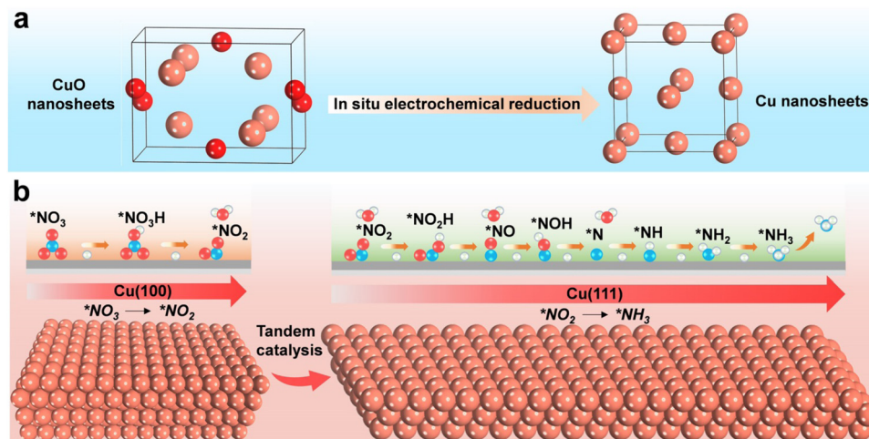
Fig. 9 Schematic illustration for enhancing the electrochemical \text{NO}_3\text{RR} over Cu nanosheets via tandem catalysis. (a) Electrochemical in situ reduction of the as-prepared CuO nanosheets during \text{NO}_3\text{RR} . (b) Tandem interaction of Cu (100) and Cu (111) facets. Reprinted with permission from ref. 100. Copyright 2023 Wiley-VCH Verlag GmbH.
