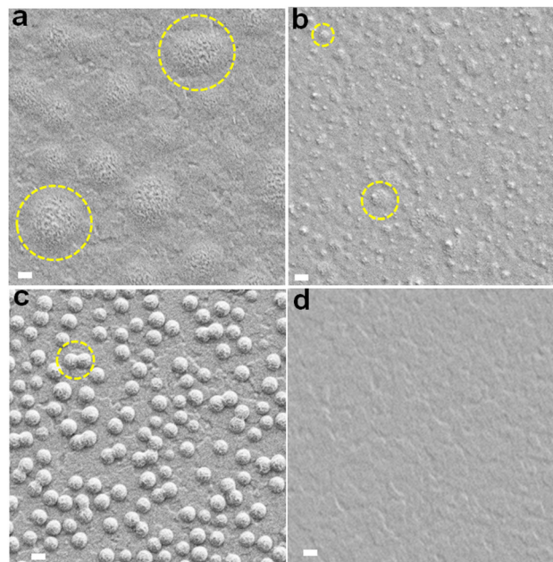
Fig. 2 SEM images ITO/bl- \text{TiO}_2 substrates after spin-coating DMF/DMSO dispersions ( 3.0 \text{mg g}^{-1} ) of (a) NG-60, (b) NG-100 and (c) NG-200 particles. An SEM of the bare ITO/bl- \text{TiO}_2 substrate is shown in (d) for comparison. The yellow circles highlight coalesced nanogels. Scale bars: 200 nm.
