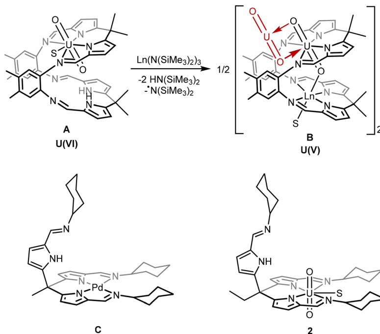
Chart 1 Top: Example of the reaction of a uranyl "Pacman" complex ( A ) and a lanthanide silylamide to form the Ln-functionalised uranyl(V) complex ( B ) via ligand deprotonation and radical transfer. 19,20 Bottom: The "hangman" palladium complex C (previous work) and uranyl complex 2 (this work) in which two ligand "arms" provide a square-planar N 4 coordination environment to the metal and the third is pendant. S indicates a THF or pyridine solvent molecule. 21,22
