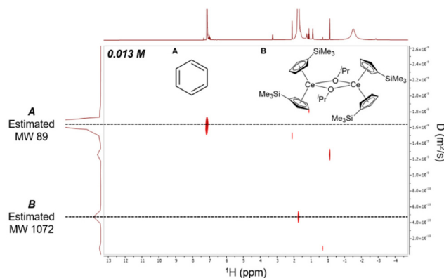
Fig. 4 2D ^1\text{H} DOSY NMR spectra of 0.013 M 2-Ce/ ^i\text{Pr} in \text{C}_6\text{D}_6 demonstrating preservation of dimer in solution.
