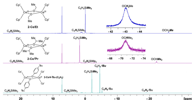
Fig. 3 ^1\text{H} NMR 298 K spectra in \text{C}_6\text{D}_6 of 2-Ce/Et, 2-Ce/ i Pr, and 2-Ce/ \text{C}_6\text{H}_4 - t Bu including insets of significantly upfield methylene and methine ^1\text{H} signals of 2-Ce/Et and 2-Ce/ i Pr, respectively.
