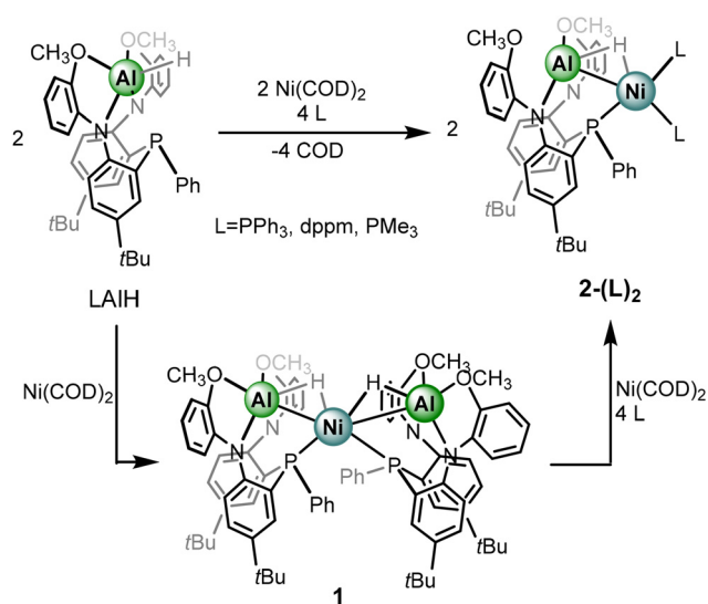
Scheme 2 Synthesis of complexes 2\text{-(L)}_2 .
