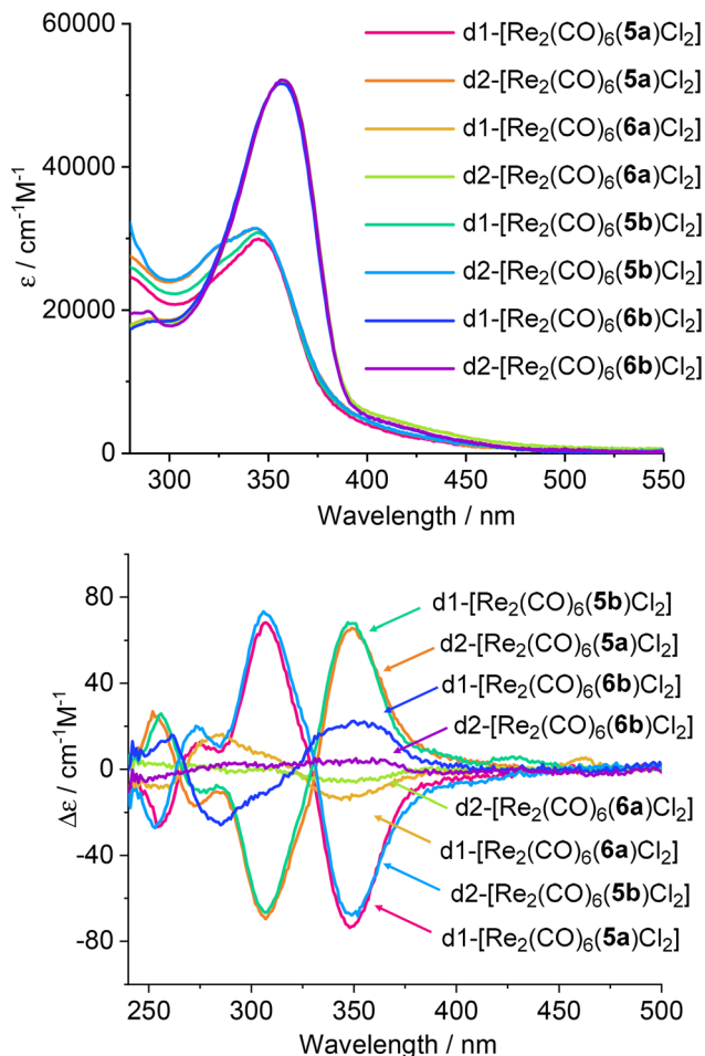
Fig. 6 UV-Vis (top) and CD (bottom) spectra of the complexes in CH 2 Cl 2 (C = 0.005 mM).
