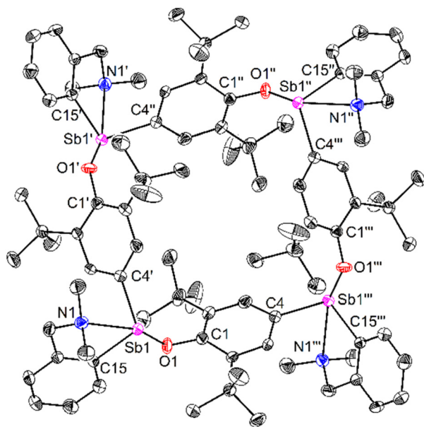
Fig. 4 Representation of the molecular structure of [\{\text{CN}^{\text{Me}_2}\text{Sb}(\text{C}_6\text{H}_2\text{-}^t\text{Bu}_2\text{-}3,5\text{-O-}4)\}_4]^{4+} ( 6a ). H atoms omitted for clarity. Ellipsoids at the 50% probability level. Selected distances (Å) and angles (°): Sb1–C4' = 2.121(5), Sb1–C15 = 2.157(4), Sb1–N1 = 2.574(4), Sb1–O1 = 2.088(4), C1–O1 = 1.346(5), C4'–Sb1–O1 = 99.36(16), C4'–Sb1–C15 = 98.36(16), C4'–Sb1–N1 = 82.47(15), C15–Sb1–N1 = 72.87(15), C15–Sb1–O1 = 84.46(15), N1–Sb1–O1 = 157.25(12).
