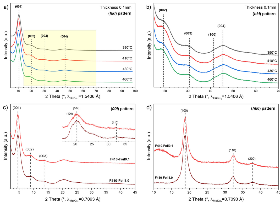
Fig. 2 (a) XRD patterns of fluorinated graphite foils ( \text{Cu K}\alpha radiation with \lambda_{\text{CuK}\alpha_1} = 1.5406 \text{ \AA} ) and (b) with magnification in the 15\text{--}70^\circ 2\theta range (shown as a yellow area on (a)). (c) and (d) are respectively the (00 l ) and ( h k0) patterns of foils of 0.1 (F410-Foil0.1, red) and 1.0 mm (F410-Foil1.0, dark red) thickness fluorinated at 390^\circ\text{C} and then annealed under \text{F}_2 gas at 410^\circ\text{C} . The latter were acquired with a \text{Mo K}\alpha source ( \lambda_{\text{MoK}\alpha_1} = 0.7093 \text{ \AA} ).
