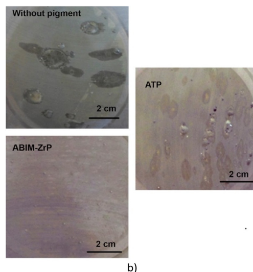
Fig. 12 (a) Impedance modulus at 10 mHz versus immersion time and (b) surface aspect after 32 days of immersion, in 0.5 M NaCl solution of zinc without or with pigment-loaded alkyd resin coating.
