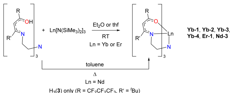
Scheme 1 (a) General synthesis and labeling scheme used for fluorinated TRAC ligands. (b) Protonolysis reactions with \text{Ln}[\text{N}(\text{SiMe}_3)_2]_3 (Ln = Nd, Er, Yb) and labeling scheme used for the prepared complexes.
