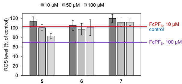
Fig. 6 Influence of compounds 5–7 on ROS generation in MDA-MB-231 (breast cancer) cells.
