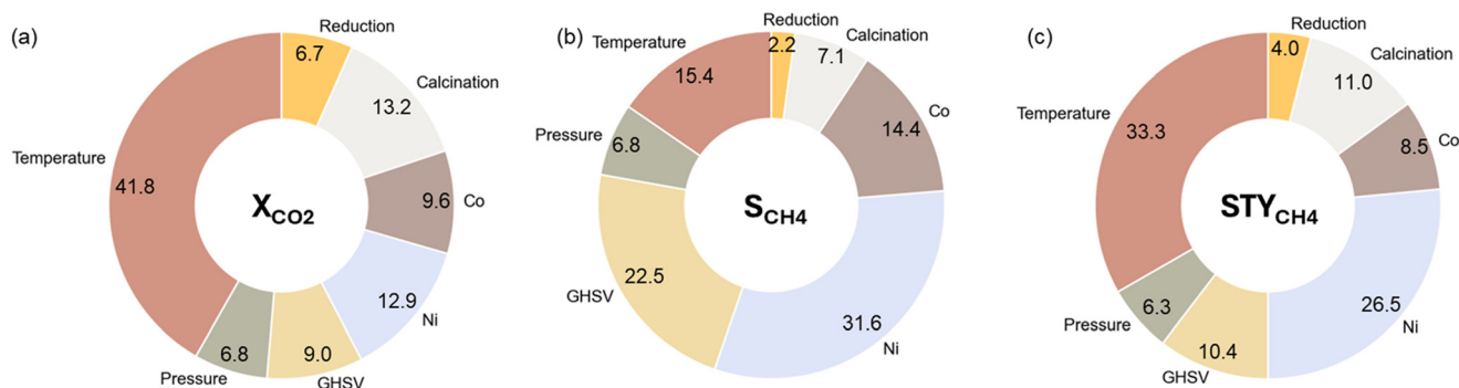
Fig. 6 Relative importance based on Shapley Additive Explanations (SHAP) values of the considered experimental variables for (a) X_{CO_2} , (b) S_{CH_4} , and (c) STY CH 4 .
