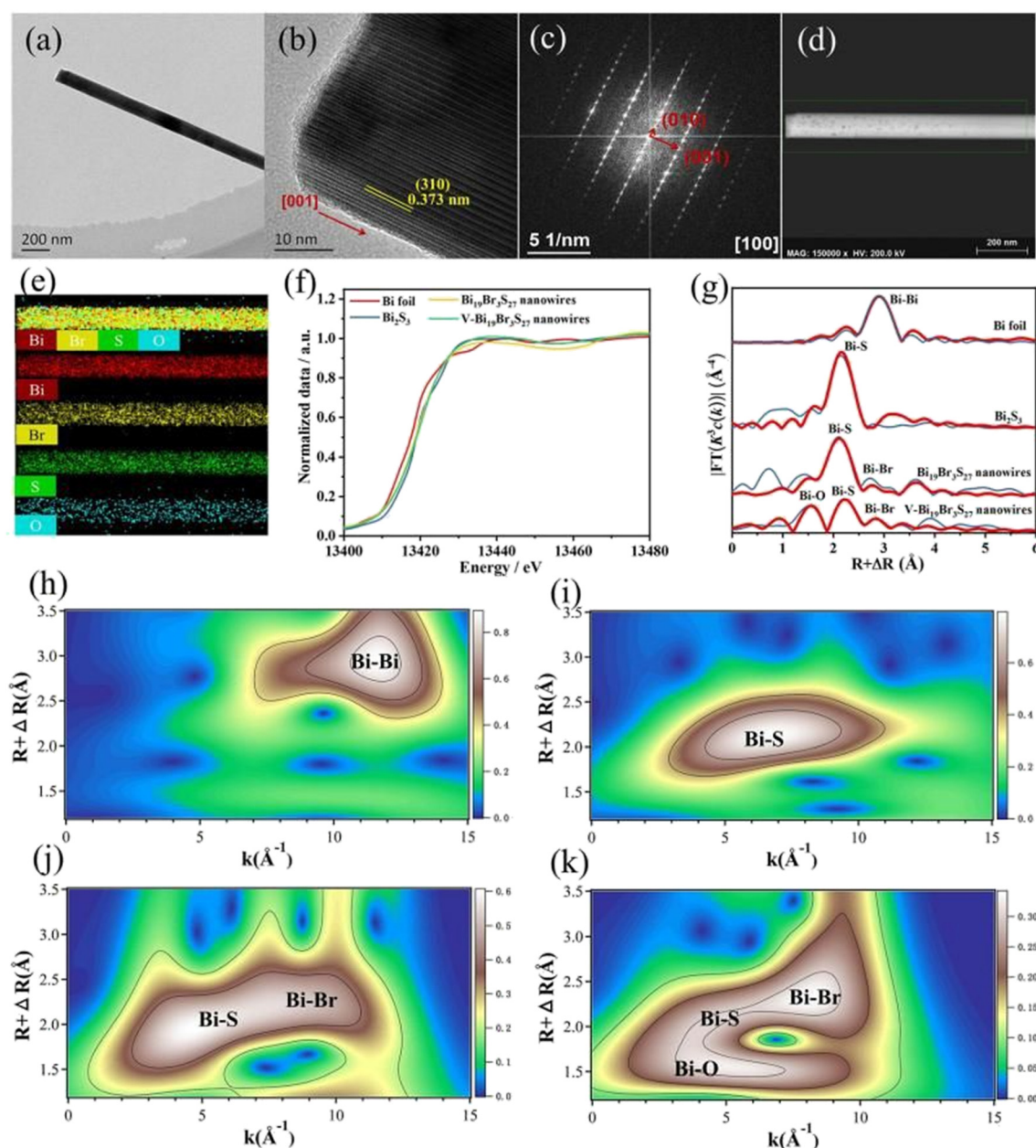
Fig. 12 (a) TEM image, (b) HRTEM image, (c) SAED image, and (d and e) EDS mapping images of a V\text{-Bi}_{19}\text{Br}_3\text{S}_{27} nanowire. (f) Bi L_{III} -edge XANES spectra of \text{Bi}_{19}\text{Br}_3\text{S}_{27} , V\text{-Bi}_{19}\text{Br}_3\text{S}_{27} nanowires and bismuth references. (g) Corresponding Fourier transforms R space fitting results. Red: observed data; blue: fitted data. (h–k) Wavelet transforms for k^2 -weighted EXAFS signals of Bi, \text{Bi}_2\text{S}_3 , \text{Bi}_{19}\text{Br}_3\text{S}_{27} , and V\text{-Bi}_{19}\text{Br}_3\text{S}_{27} , respectively. 54
