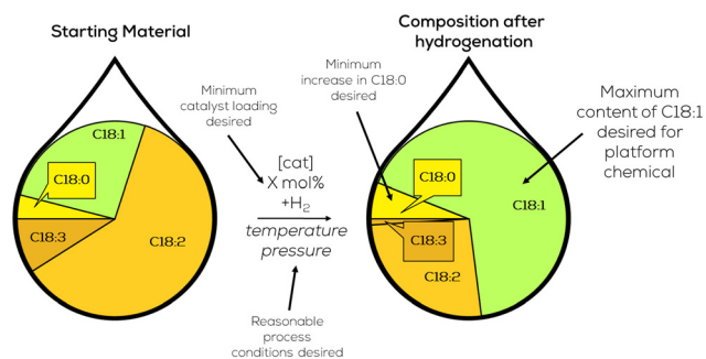
Fig. 8 Example for the evaluation of the given catalytic hydrogenation reaction.
