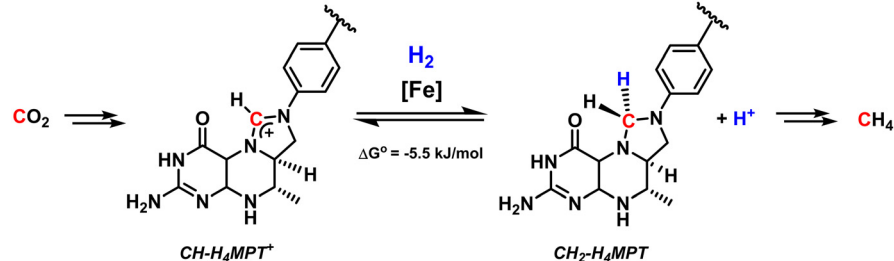
Scheme 4 Structure of the [Fe]-hydrogenase metalloenzyme and the FeGP cofactor (top). Catalytic hydrogenation by [Fe]-hydrogenase in the biological methanogenesis (bottom).
