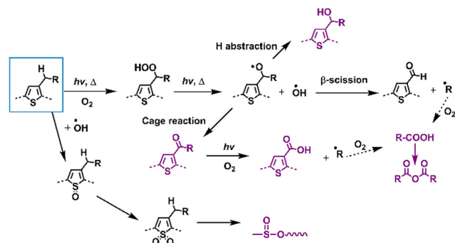
Fig. 17 Photodegradation mechanisms (with O_2 ) of classic D-type polymer donors – poly(thiophene) derivatives. 136–139,141,142
