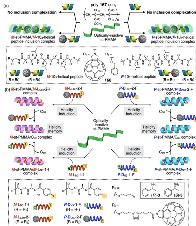
Fig. 84 (a) Schematic illustration of the asymmetry induction of PMMA poly-167 upon encapsulation of fullerenes derivatives functionalized with P or M 3_{10} -helical peptide (168) or with (b) P or M polylactic acid. Reproduced from ref. 424 with permission from the American Chemical Society, copyright 2020.
